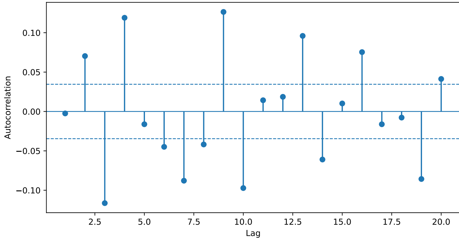
Dataset 3 - ACF of HAR-MA(1) innovations
